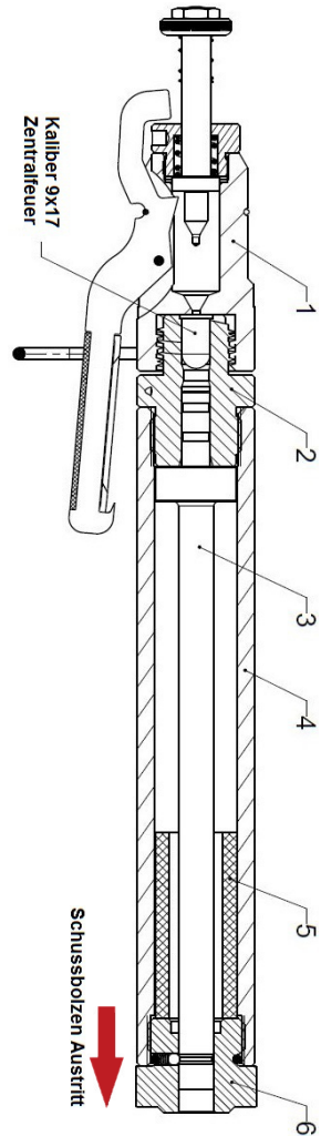
fig.: captive bolt stunner Bullen Blitz (loaded and tensioned)
